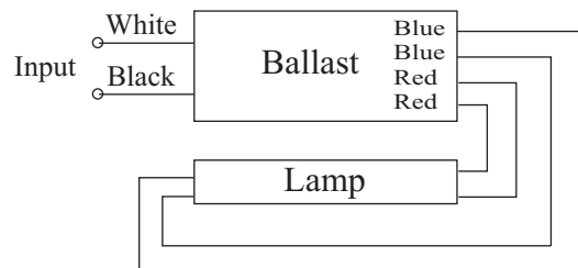
Ballast Wiring Diagram
