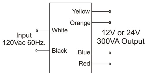
Output wiring option #2 (One 12V 300VA Branch)
